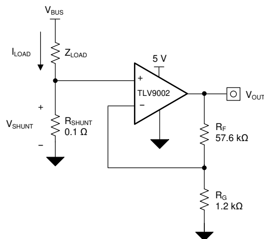
图 9-1. TLV900x in a Low-Side, Current-Sensing Application
