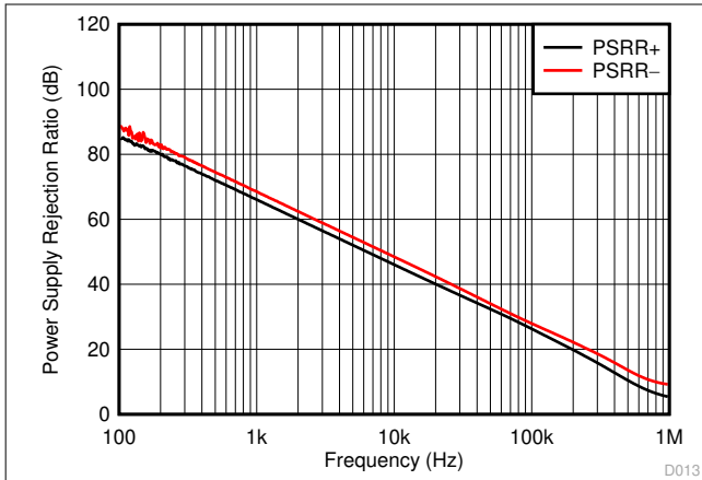
图 7-13. PSRR vs Frequency
