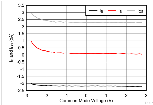
图 7-7. I_B and I_{OS} vs Common-Mode Voltage
