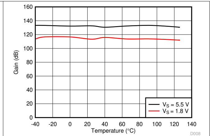
图 7-8. Open-Loop Gain vs Temperature
