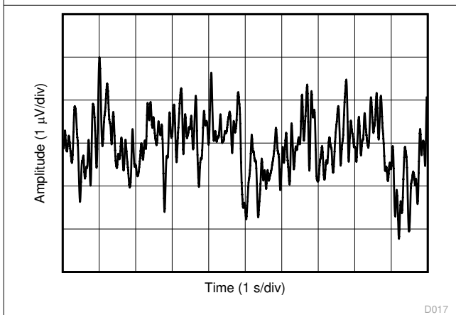
图 7-17. 0.1-Hz to 10-Hz Integrated Voltage Noise
