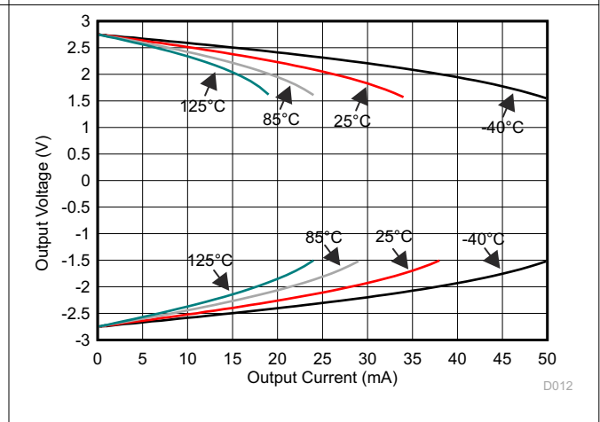
图 7-12. Output Voltage vs Output Current (Claw)
