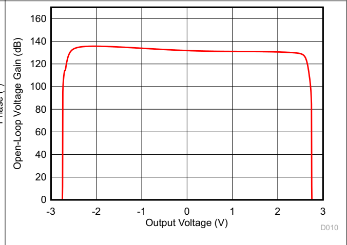
图 7-10. Open-Loop Gain vs Output Voltage
