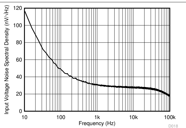
图 7-18. Input Voltage Noise Spectral Density
