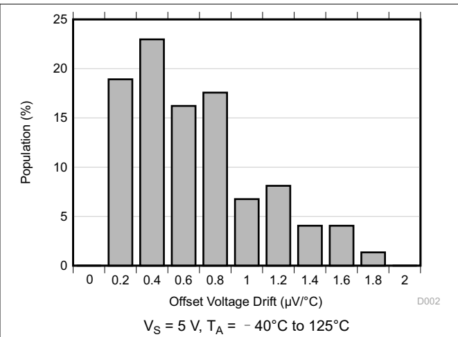
图 7-2. Offset Voltage Drift Distribution Histogram
