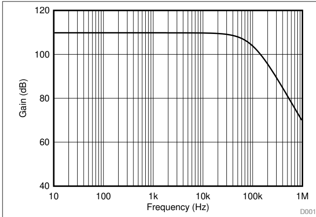
图 9-4. Photodiode Amplifier Circuit AC Gain Results
